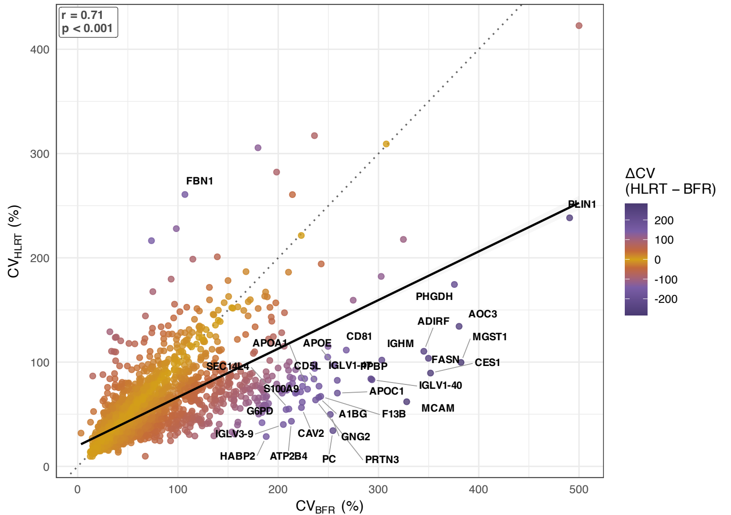
Per-protein CV by group
