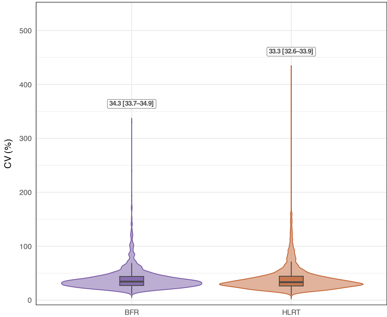
Per-protein CV by group
