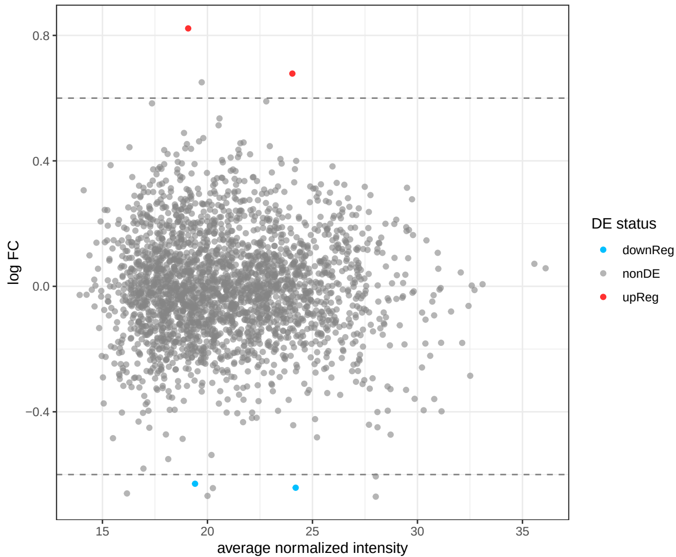
Training_BFR, adjusted p-value
