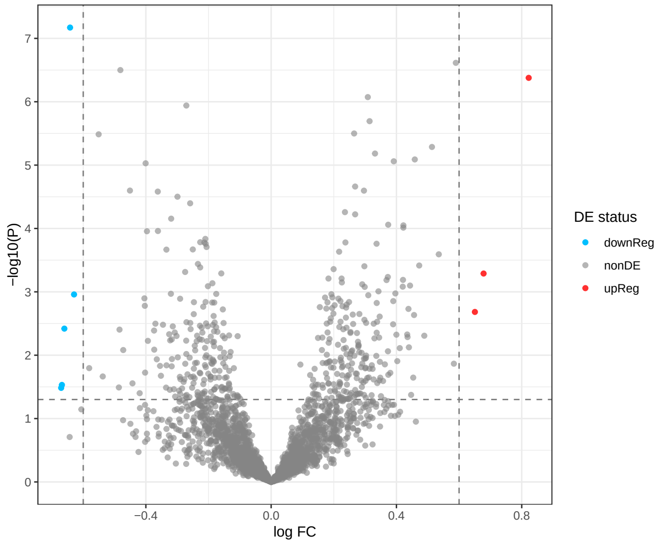
Training_BFR, raw p-value
