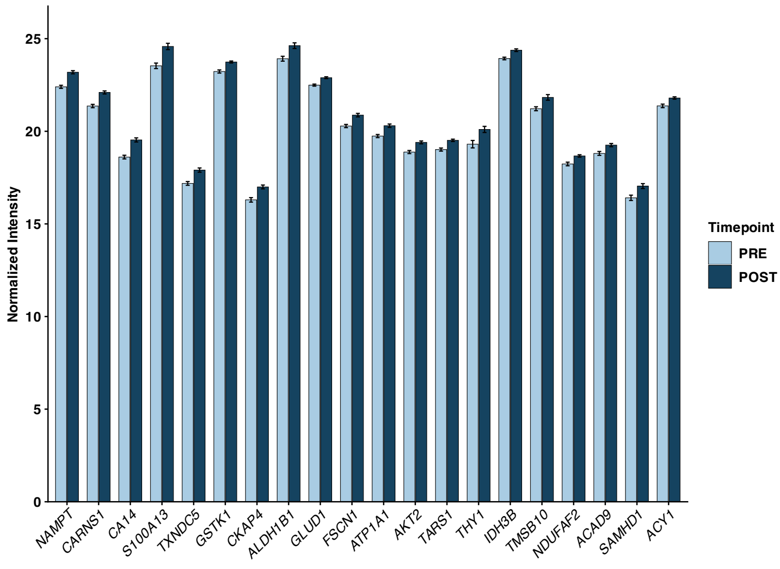
Training_HLRT — HLRT_POST vs HLRT_PRE (Top 20, UP-regulated)
