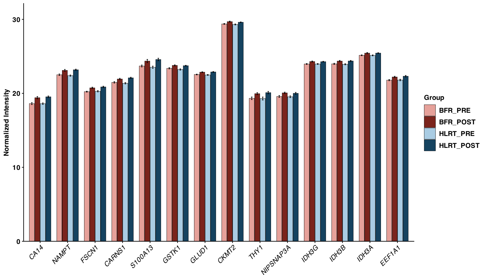
Concordant UP-regulated — Significant in Both Contrasts (Top 14)
