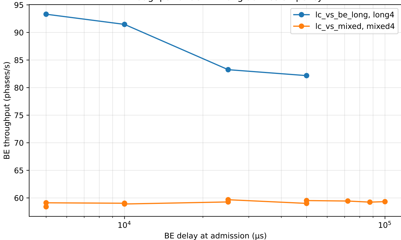
BE throughput under BE-long admission policy
