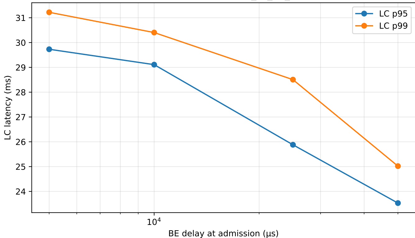
LC tail latency under policy: lc_vs_be_long, long4
