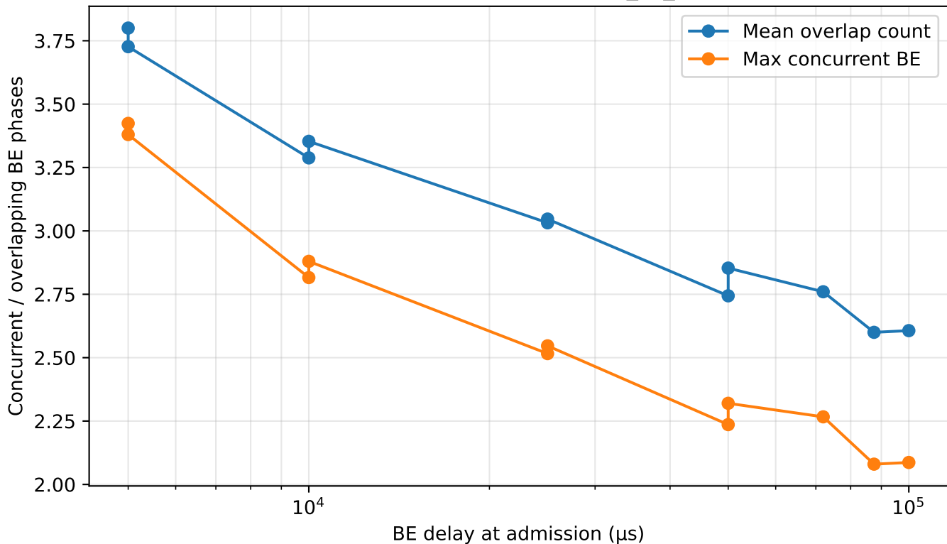
BE concurrency during LC requests: lc_vs_mixed, mixed4
