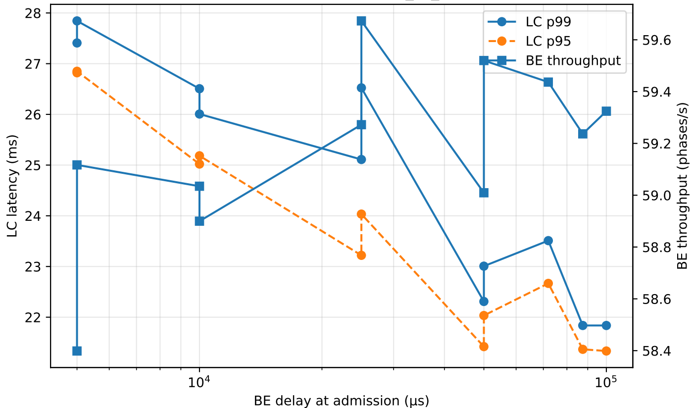
LC tail latency vs BE throughput: lc_vs_mixed, mixed4
