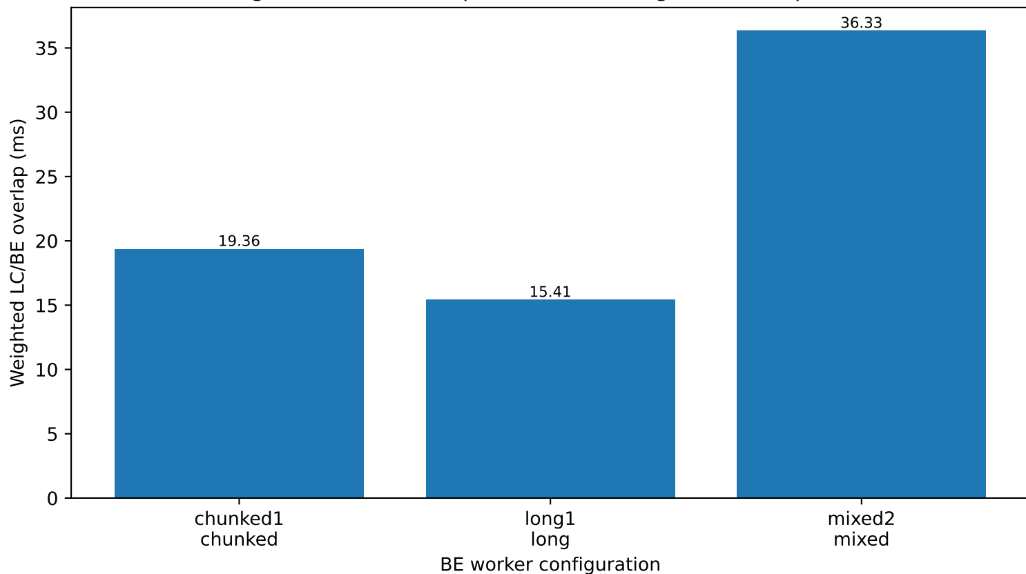
Weighted LC/BE overlap under increasing BE worker pressure
