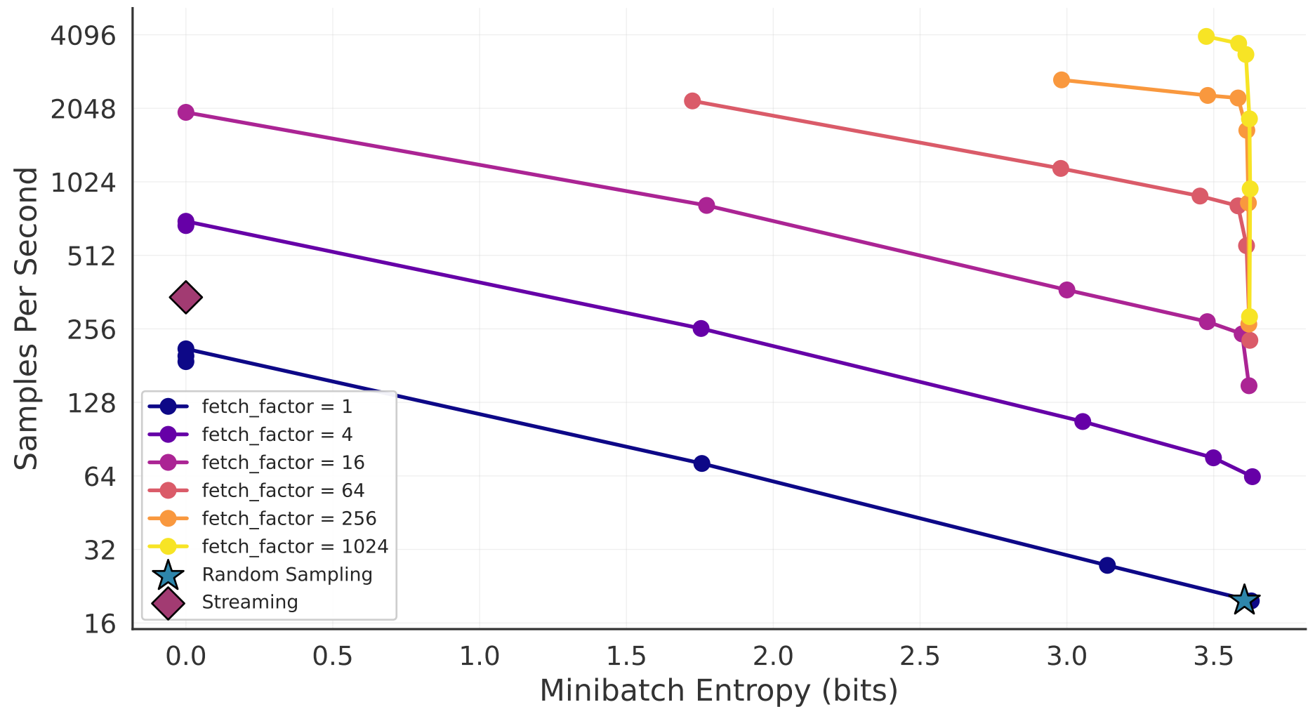
Throughput vs Minibatch Entropy Tradeoff
