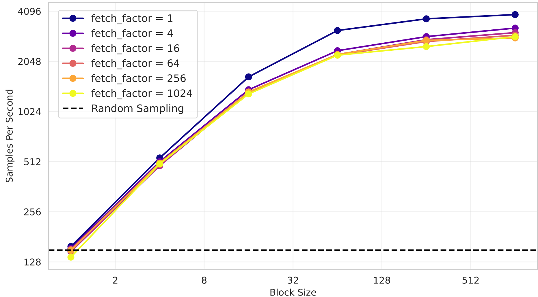
scDataset Throughput with HuggingFace
