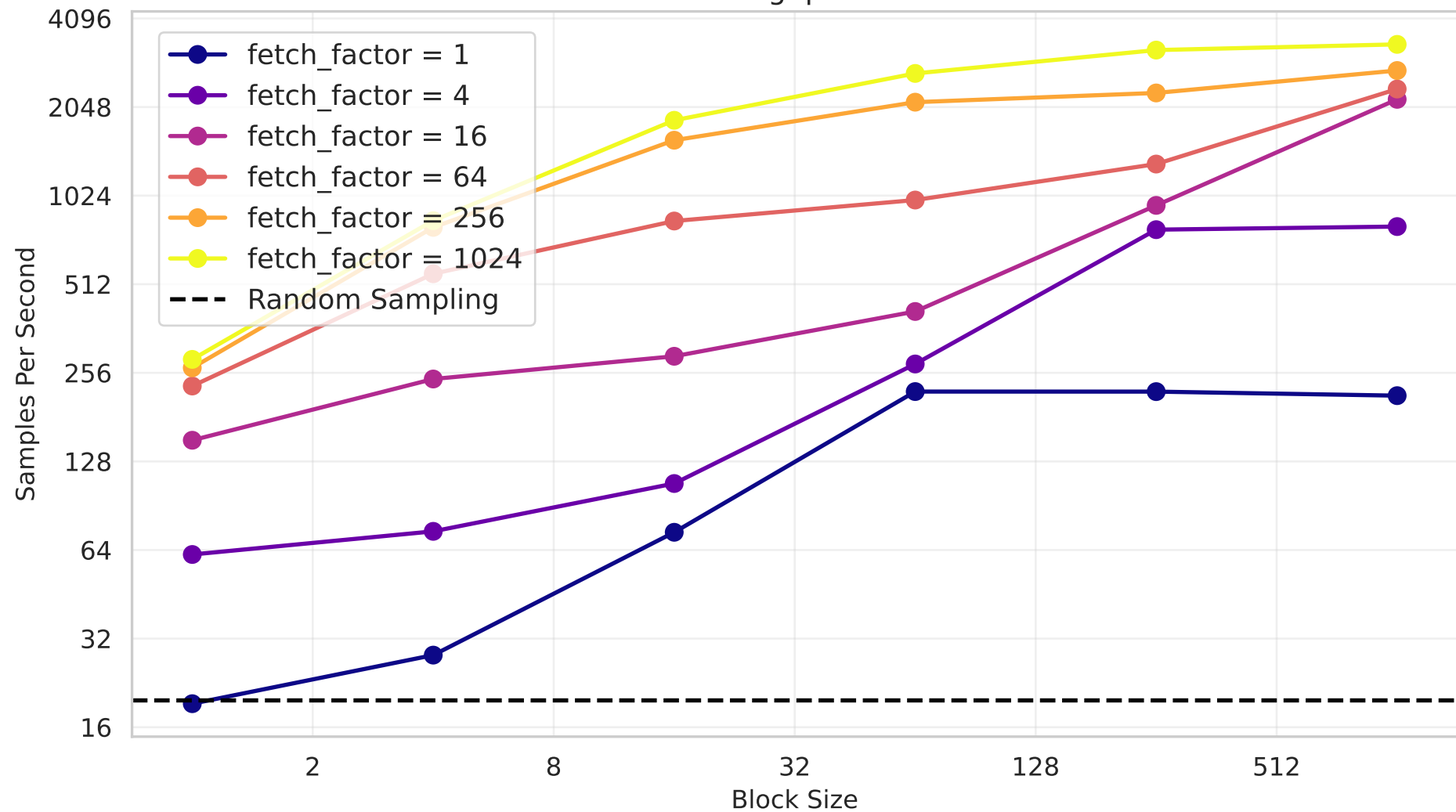
scDataset Throughput with AnnData
