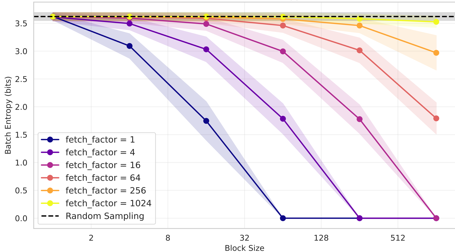
scDataset Batch Entropy
