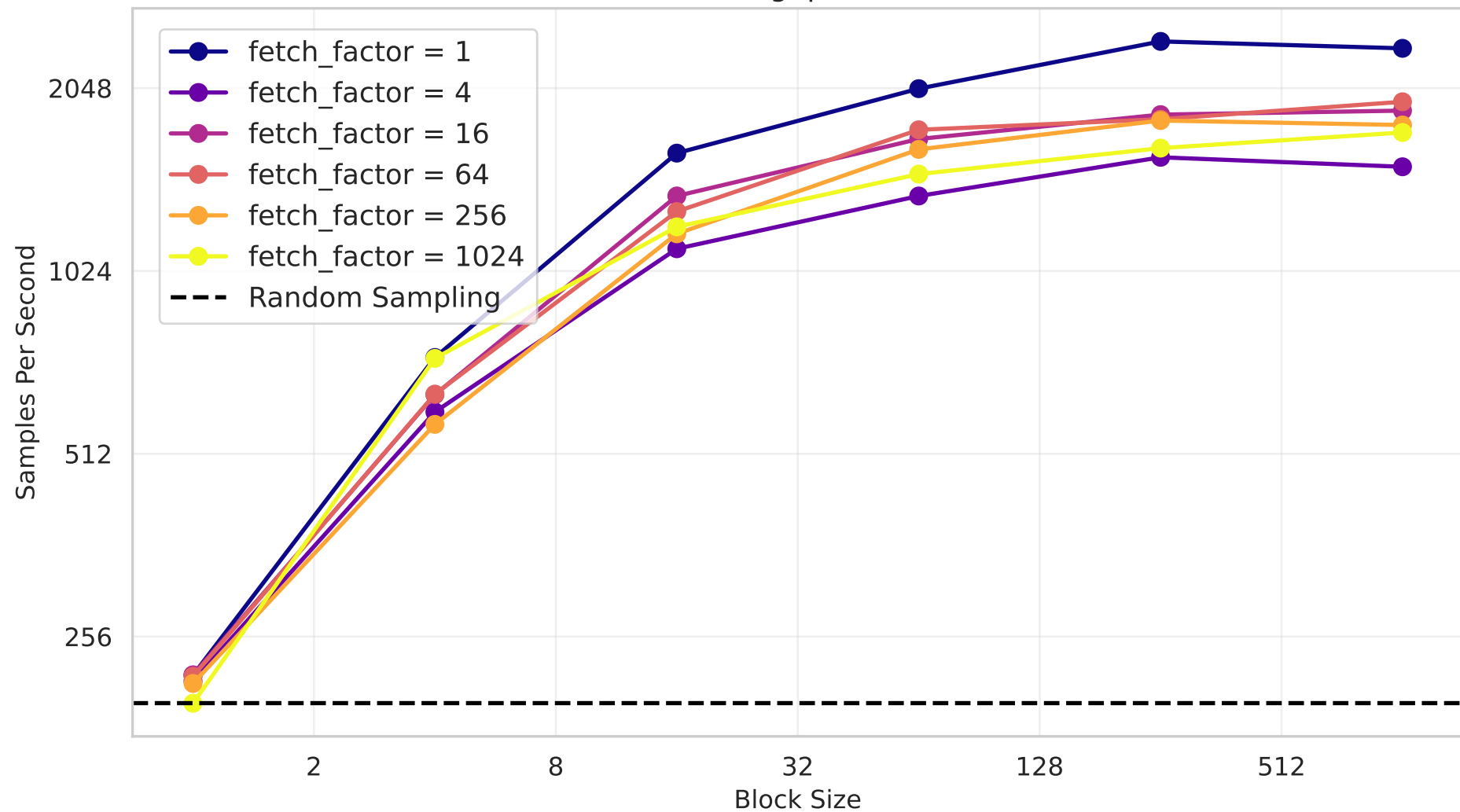
scDataset Throughput with BioNeMo
