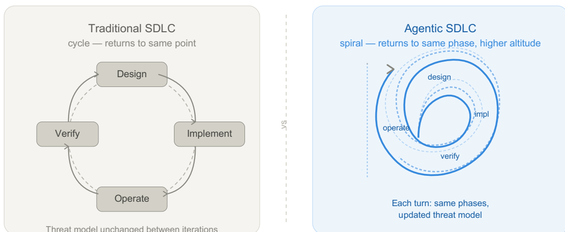
Figure 1: Traditional SDLC returns to the same point. Agentic SDLC returns to the same phase at a higher altitude — with changed system, changed tool surface, and updated threat model. Governance spans every turn of the spiral rather than appearing as a single step.
