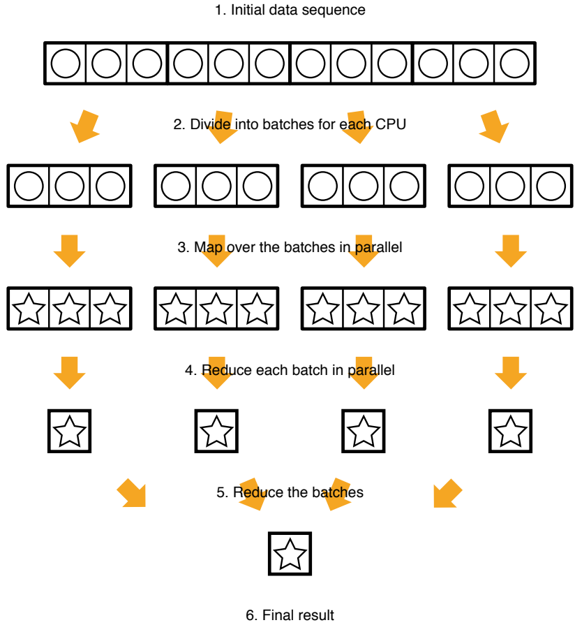
Figure 18.4: parallelFoldMap algorithm
