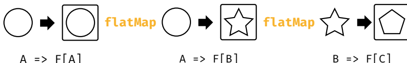
Figure 19.9: Sequencing monadic transforms
