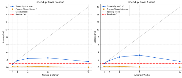
Figure 6. Speedup "email presenti" e "email assenti"
