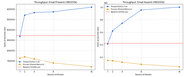
Figure 9. Throughput "email presenti" e "email assenti"
