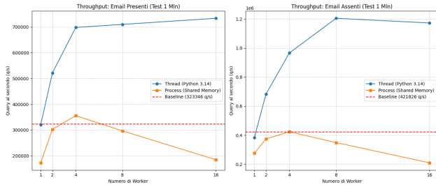
Figure 11. Throughput "email presenti" e "email assenti"
