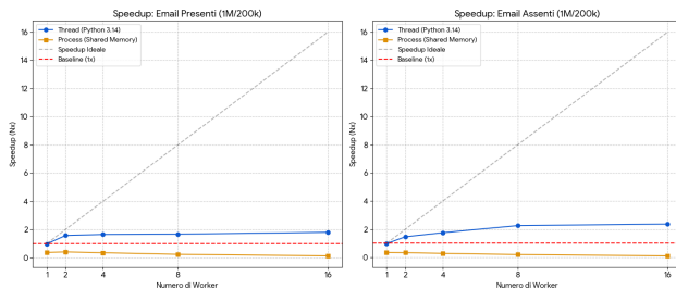
Figure 8. Speedup "email presenti" e "email assenti"
