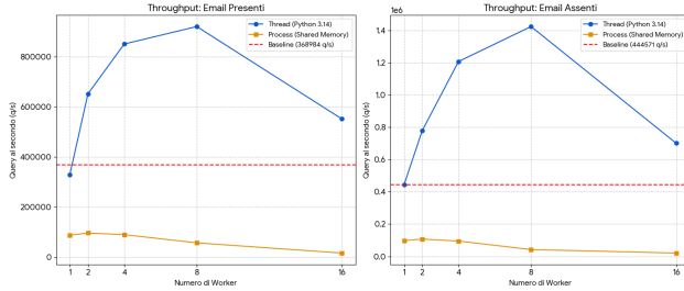
Figure 7. Throughput "email presenti" e "email assenti"
