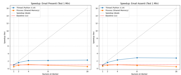
Figure 10. Speedup "email presenti" e "email assenti"
