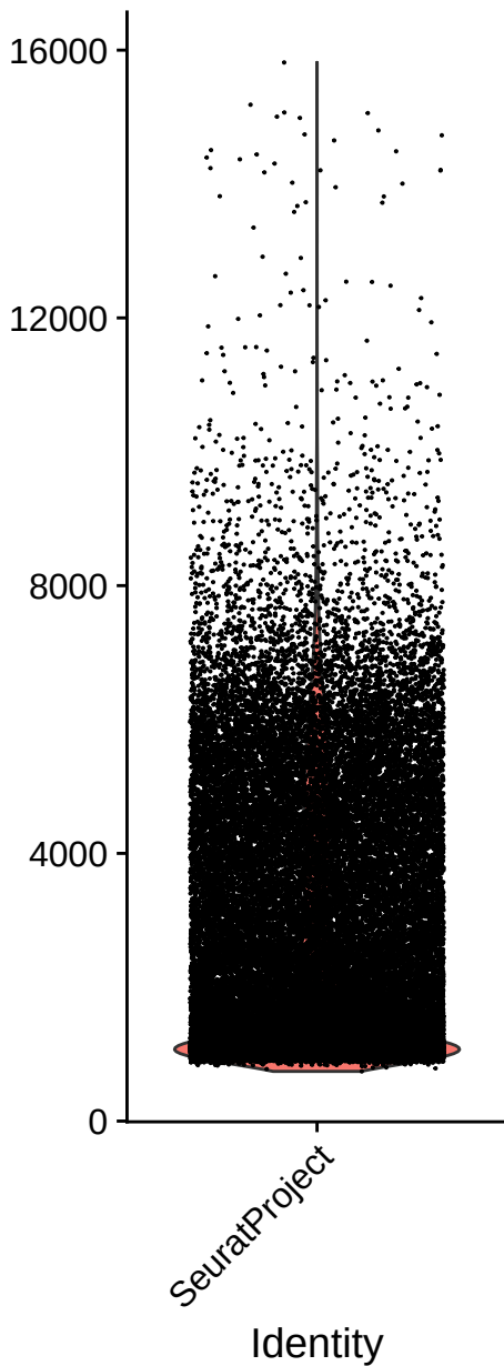
nFeature_RNA
