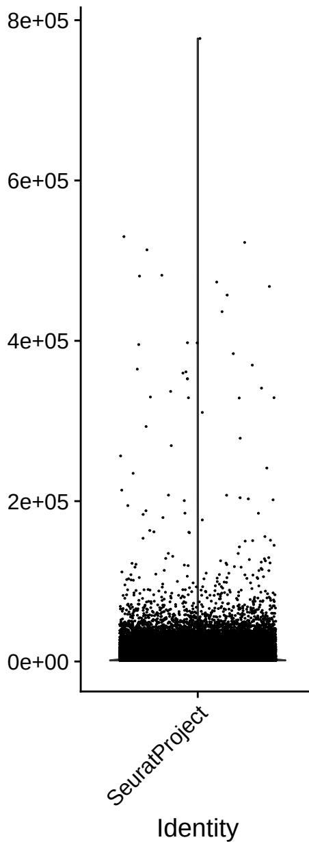
nCount_RNA
