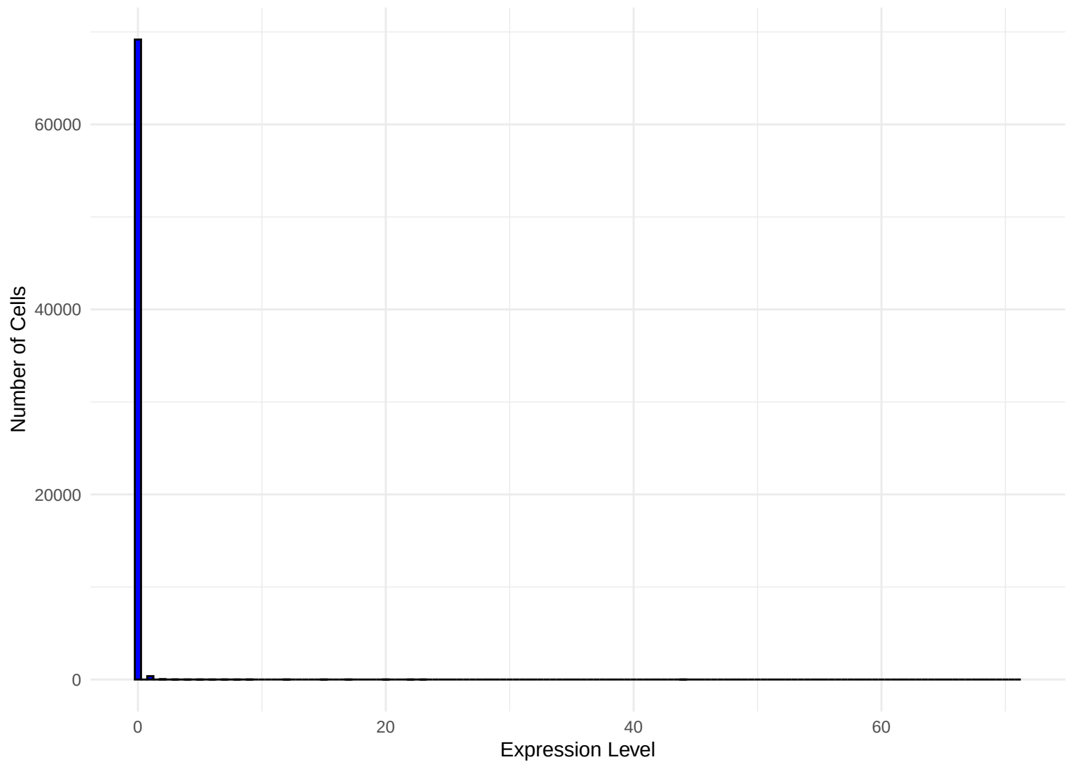
Oxt Expression (RNA Counts)
