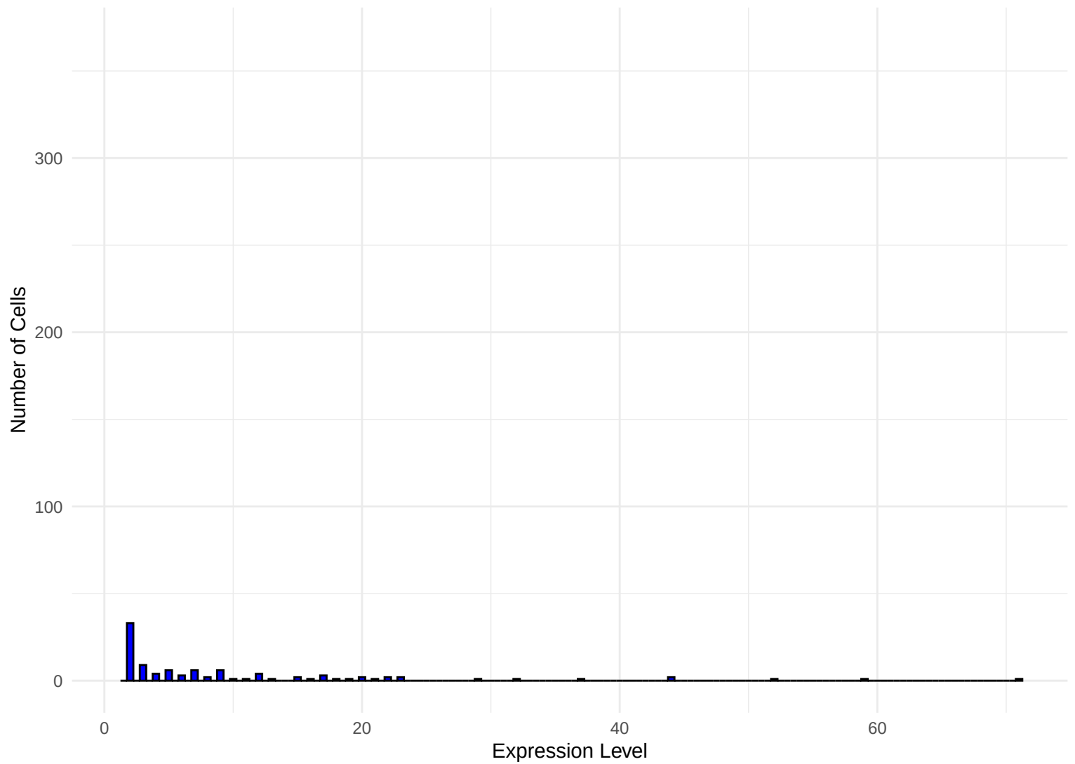
Oxt Expression (RNA Counts)
