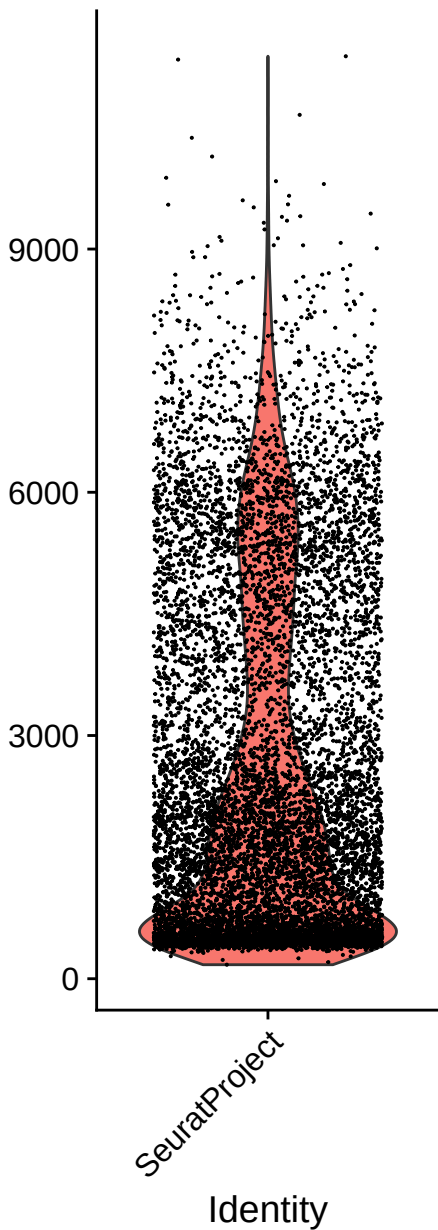
nFeature_RNA
