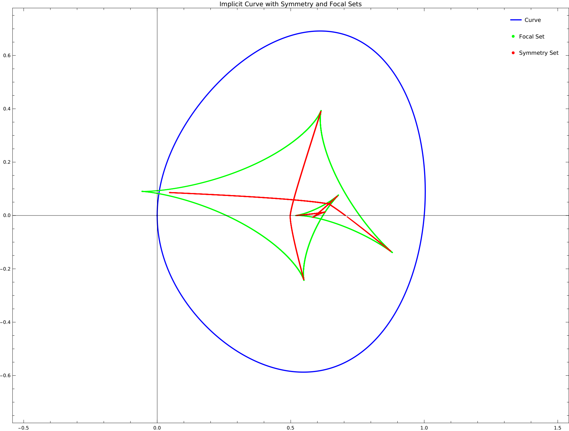
Implicit Curve with Symmetry and Focal Sets
