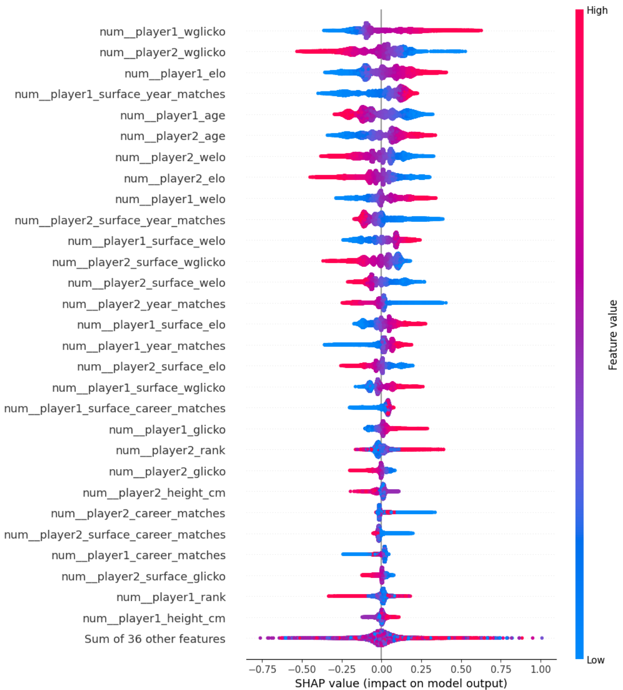
Figure 7: A beeswarm plot showing how the top features in a dataset impact the CatBoost model output.
