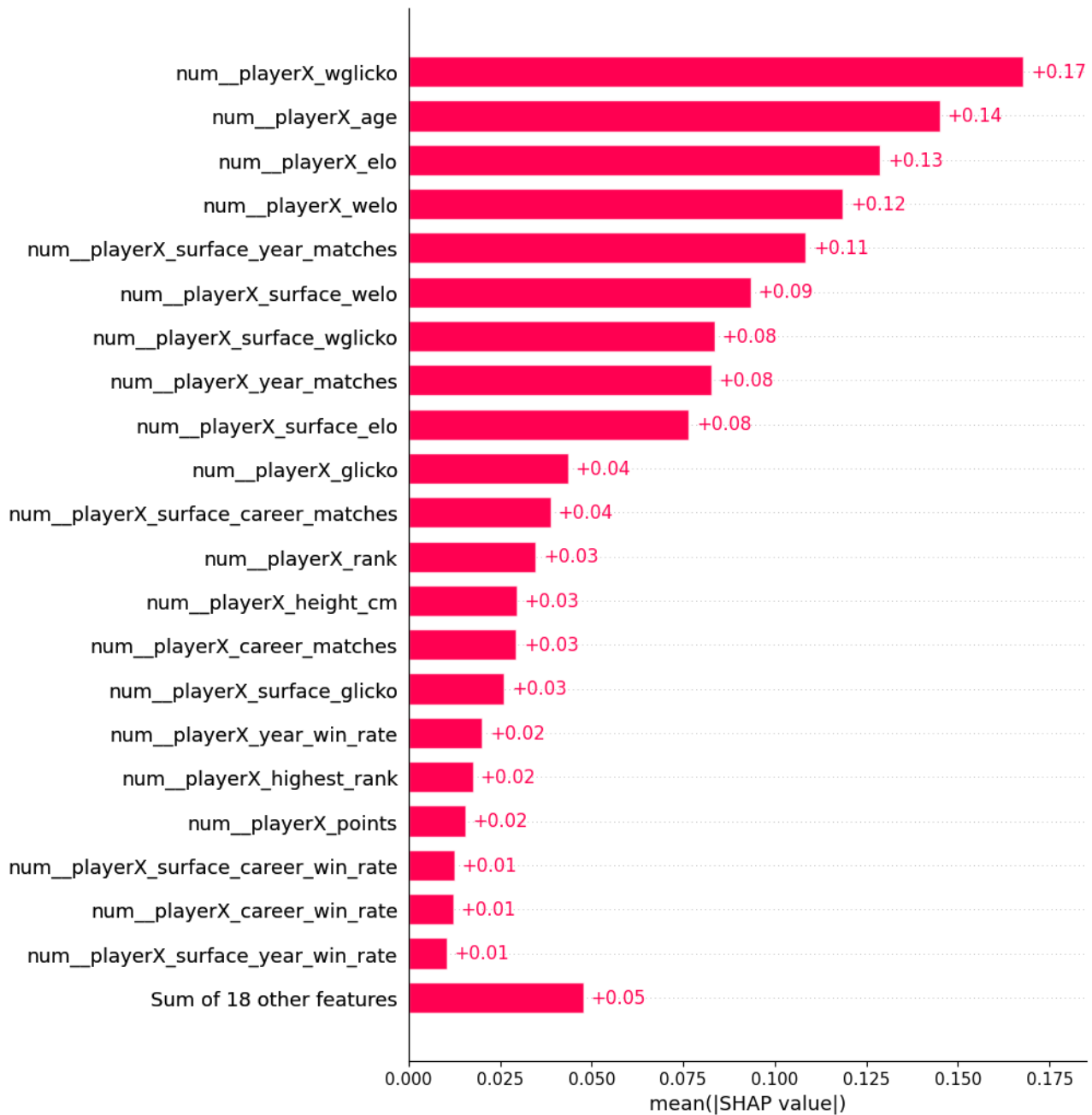
Figure 8: A bar chart showing how the top grouped features in a dataset impact the CatBoost model output (most important features first).
