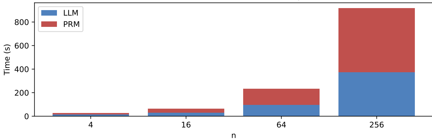
LLM + PRM Time Breakdown by n
