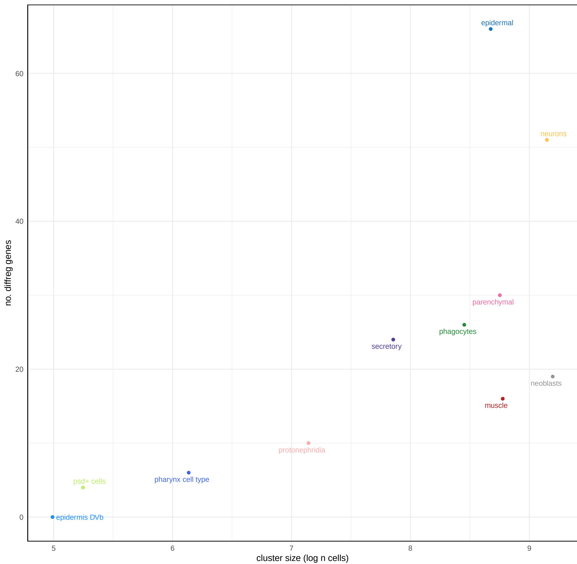
Cluster size vs # DiffReg lhx1/5-1(RNAi)
