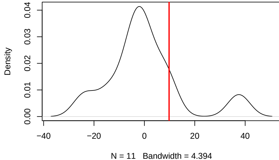
density.default(x = sero_lhx_lm$residuals)
