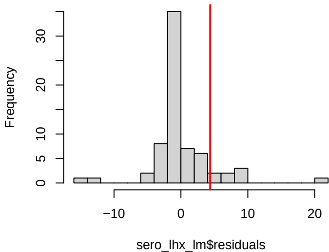
Histogram of sero_lhx_lm$residuals
