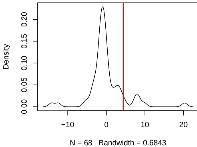
density.default(x = sero_lhx_lm$residuals)
