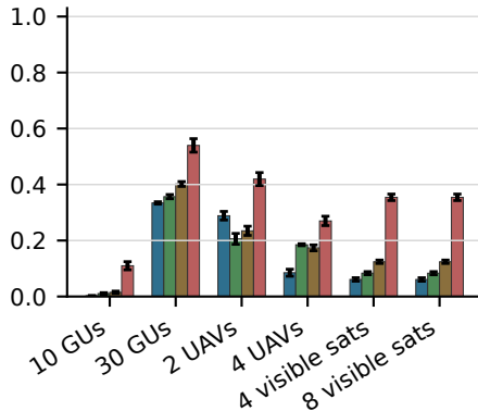
Drop ratio
