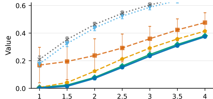
Drop ratio
