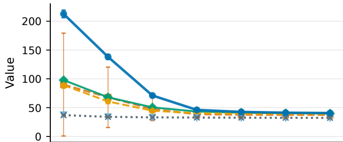
Reward
