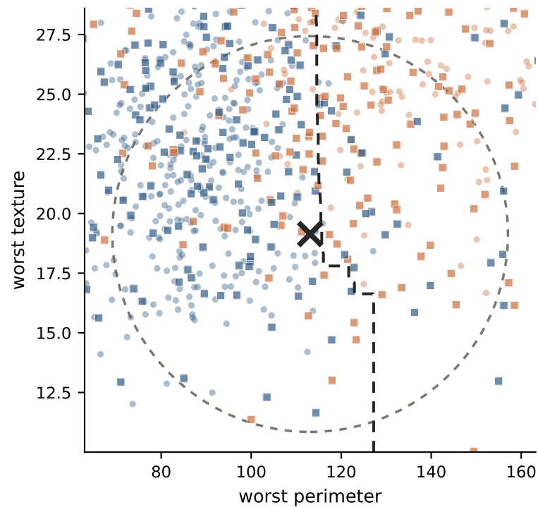
D · predictions on the neighbors
