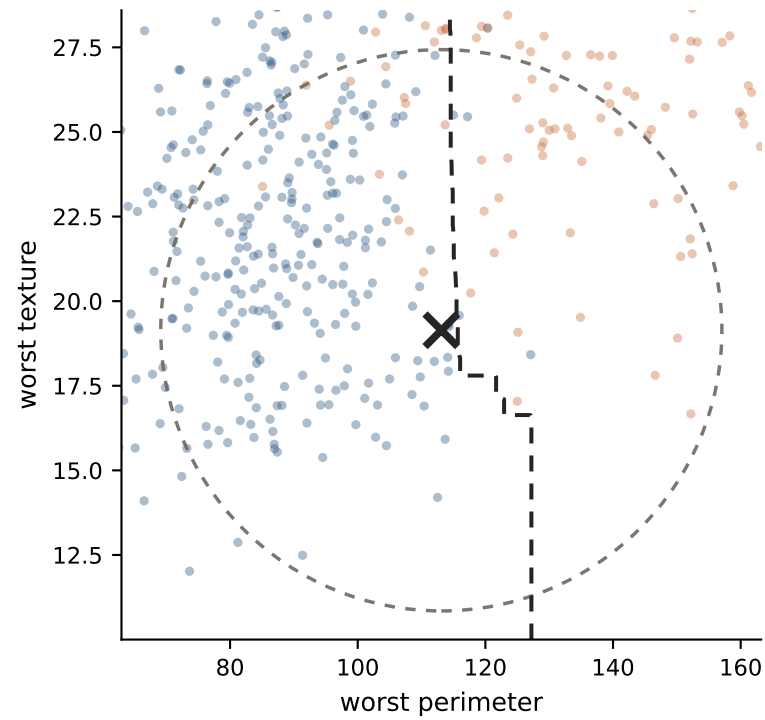
B · the local neighborhood
