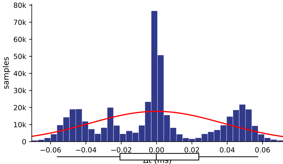
Insecure (No Encryption) Std = 0.038 ms
