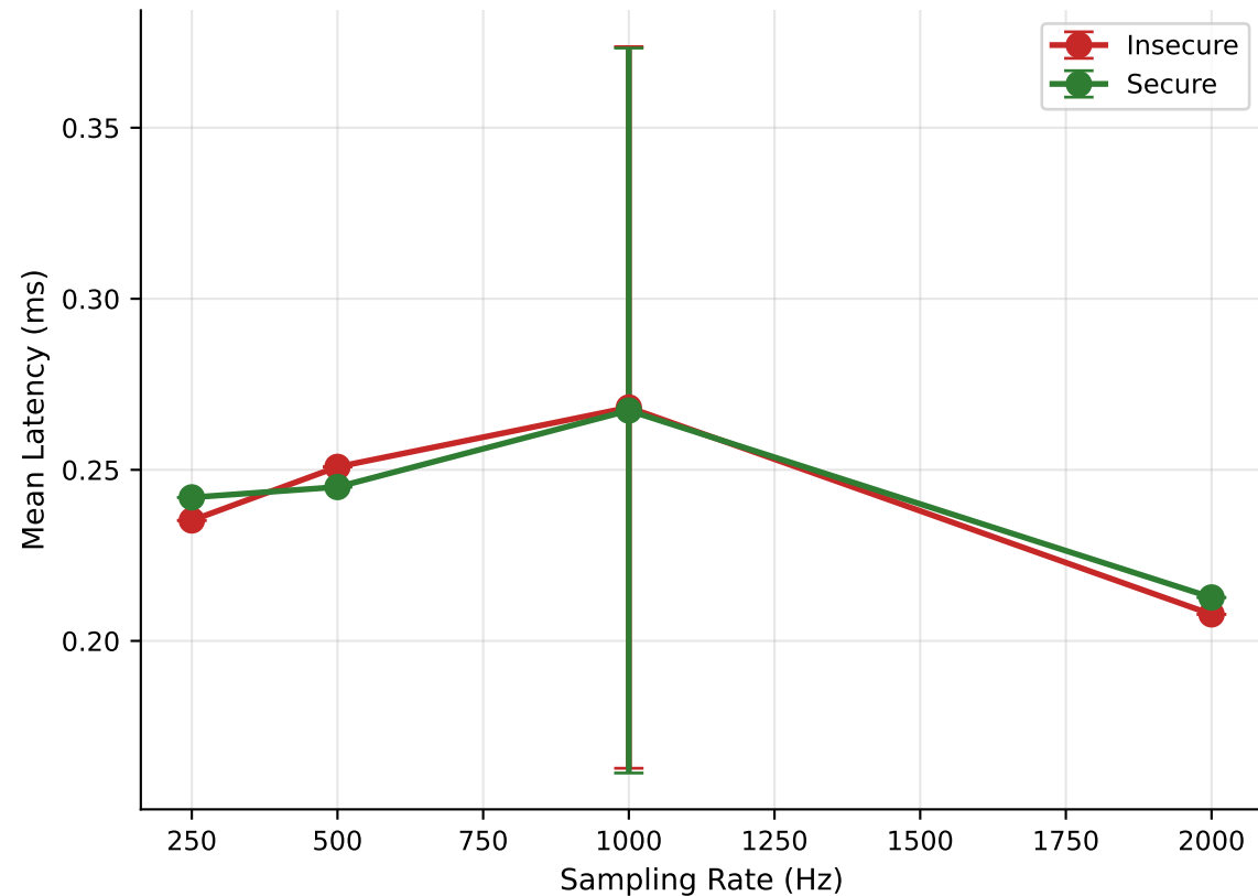
Latency vs Sampling Rate
