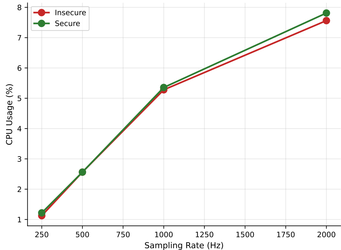
CPU Usage vs Sampling Rate
