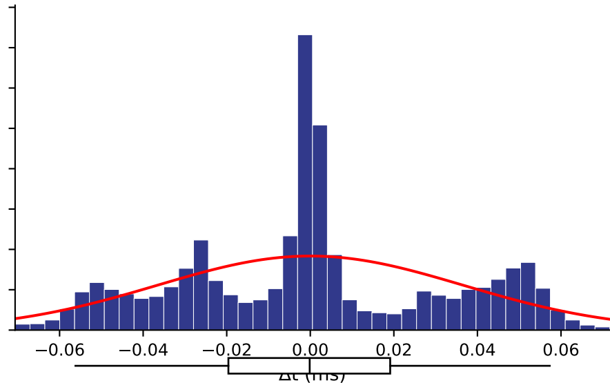
Secure (Encrypted) Std = 0.037 ms
