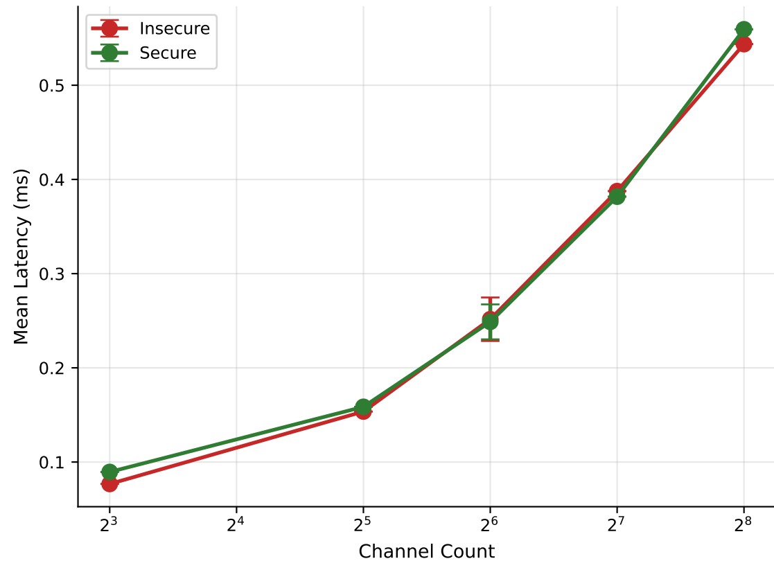
Latency vs Channel Count
