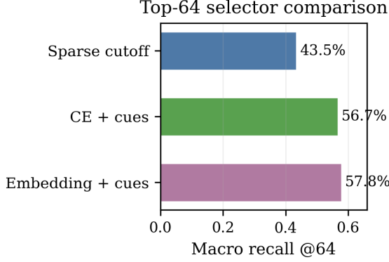
Figure 2: Embedding plus factual cues is the best top-64 selector. It reaches 57.8% macro recall, above sparse cutoff and cross-encoder-plus-cue variants, justifying its use for the classifier evidence context.
