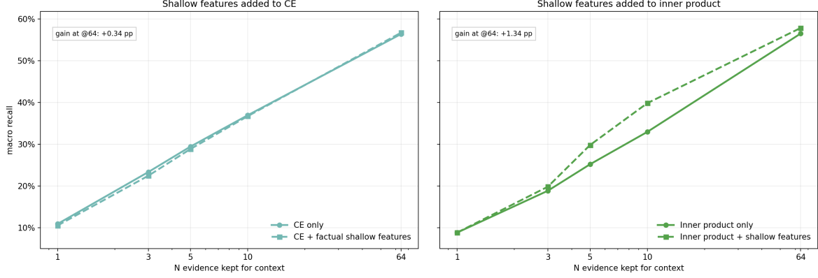
Figure 4: Factual cues preserve or improve semantic ranking. The gain is small for the already strong cross-encoder but clearer for embedding inner product, supporting feature fusion rather than a purely semantic context selector.
