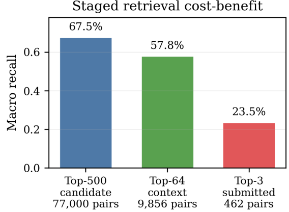
Figure 1: Staged pruning keeps recall while reducing pair count. The candidate and reranked-context pools retain most recoverable evidence while avoiding the orders-of-magnitude cost of full-corpus neural scoring, which would require about 186 million claim–evidence pairs on the development split.
