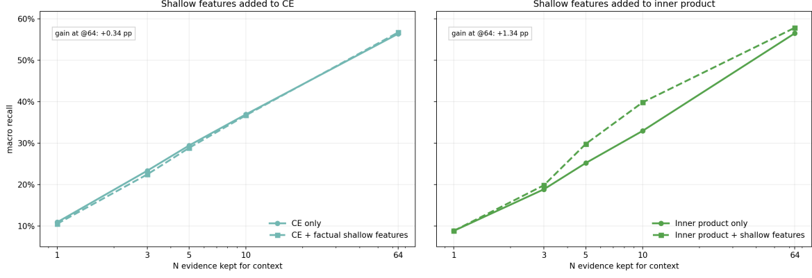
Figure 5: Factual cues preserve or improve semantic ranking. Gains are small for the strong cross-encoder but clearer for embedding inner product, supporting feature fusion over a purely semantic selector.
