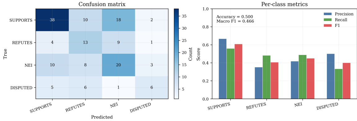
Figure 6: Classifier errors concentrate among the three main labels. The final Colab run is strongest on SUPPORTS; DISPUTED remains hard because it is rare and often evidence-conflict dependent.
