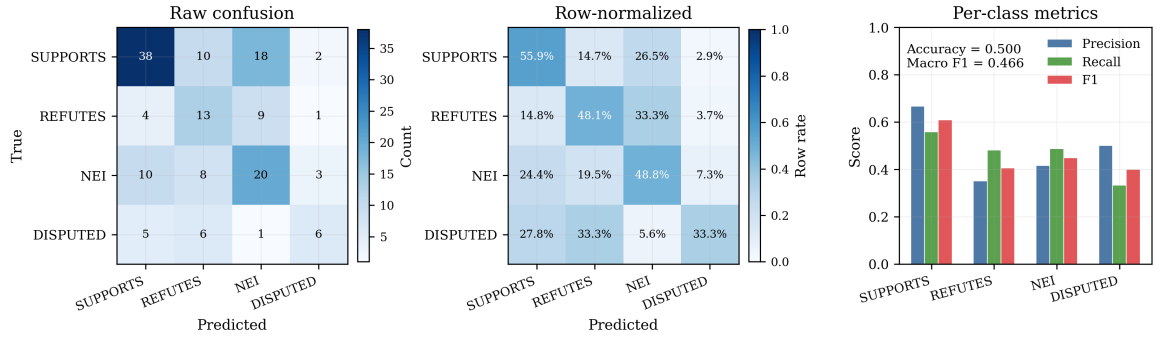
Figure 7: Classifier diagnostics. Raw counts show total error mass, row-normalized confusion controls for class support, and per-class precision/recall/F1 summarizes the classification report.
