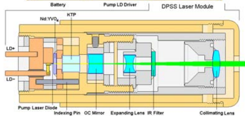
Edmund Scientific L54-101 Green DPSS Laser Pointer
