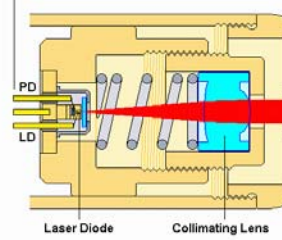
Typical Red Laser Pointer
