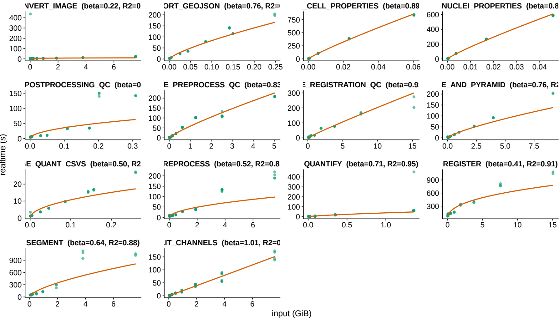
Runtime scaling per process (power law) Linear axes; curve = fitted power law. \beta = log-log slope (1 = linear, >1 super-linear, <1 sub-linear).
