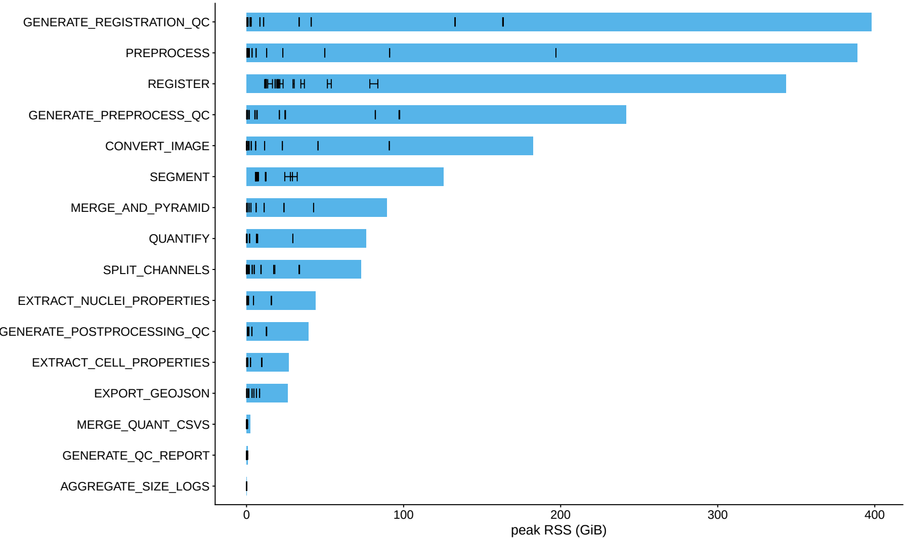
Peak RSS by process (mean +/- sd across repeats)
