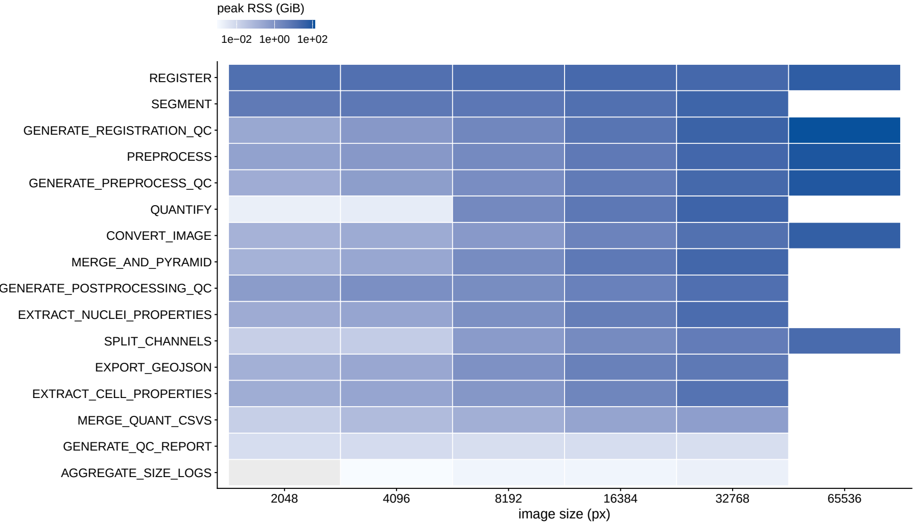
Where the memory goes Peak RSS by stage x image size (log colour). Darker = the memory bottleneck at that size.
