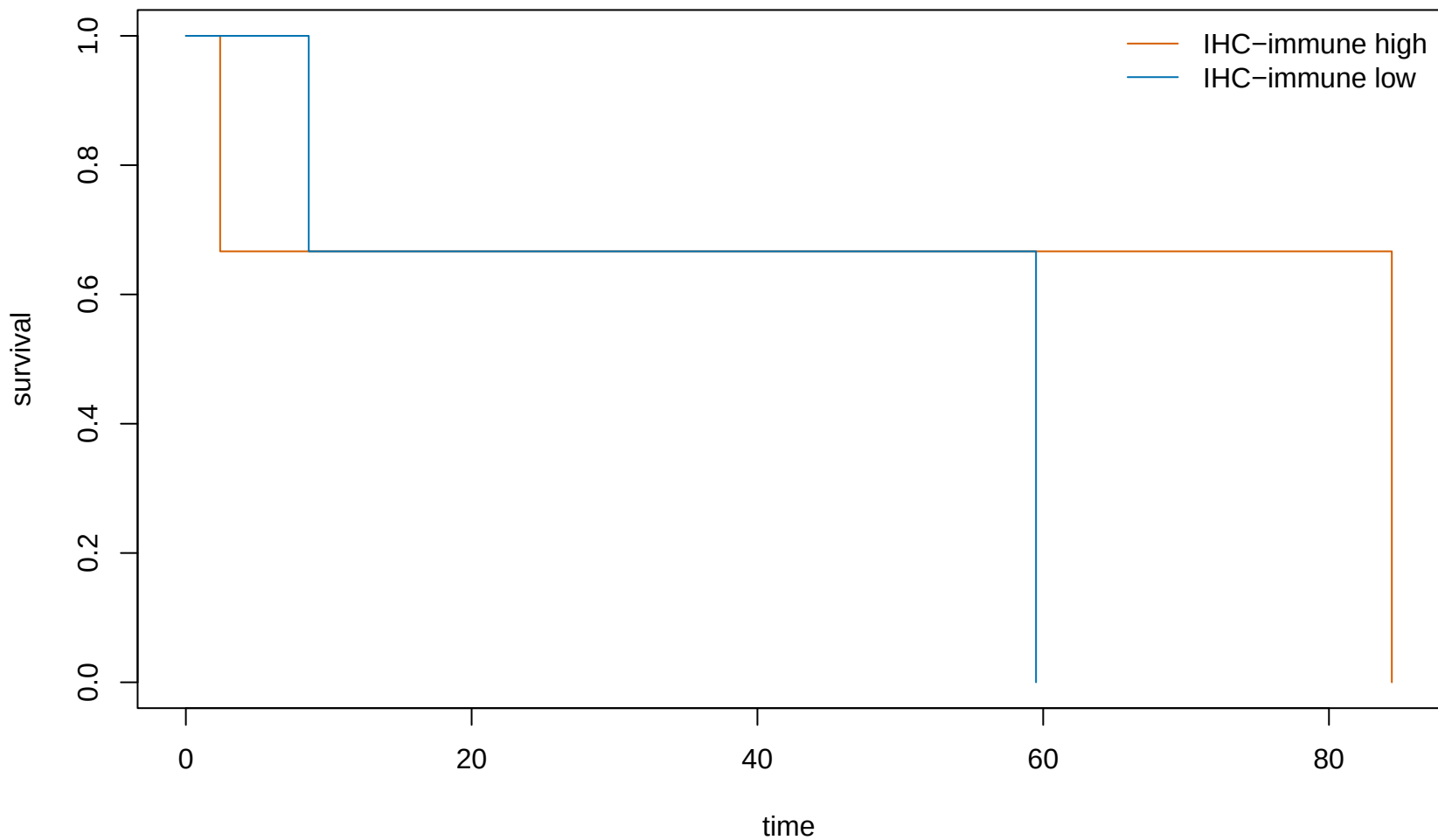
OS by IHC immune score
