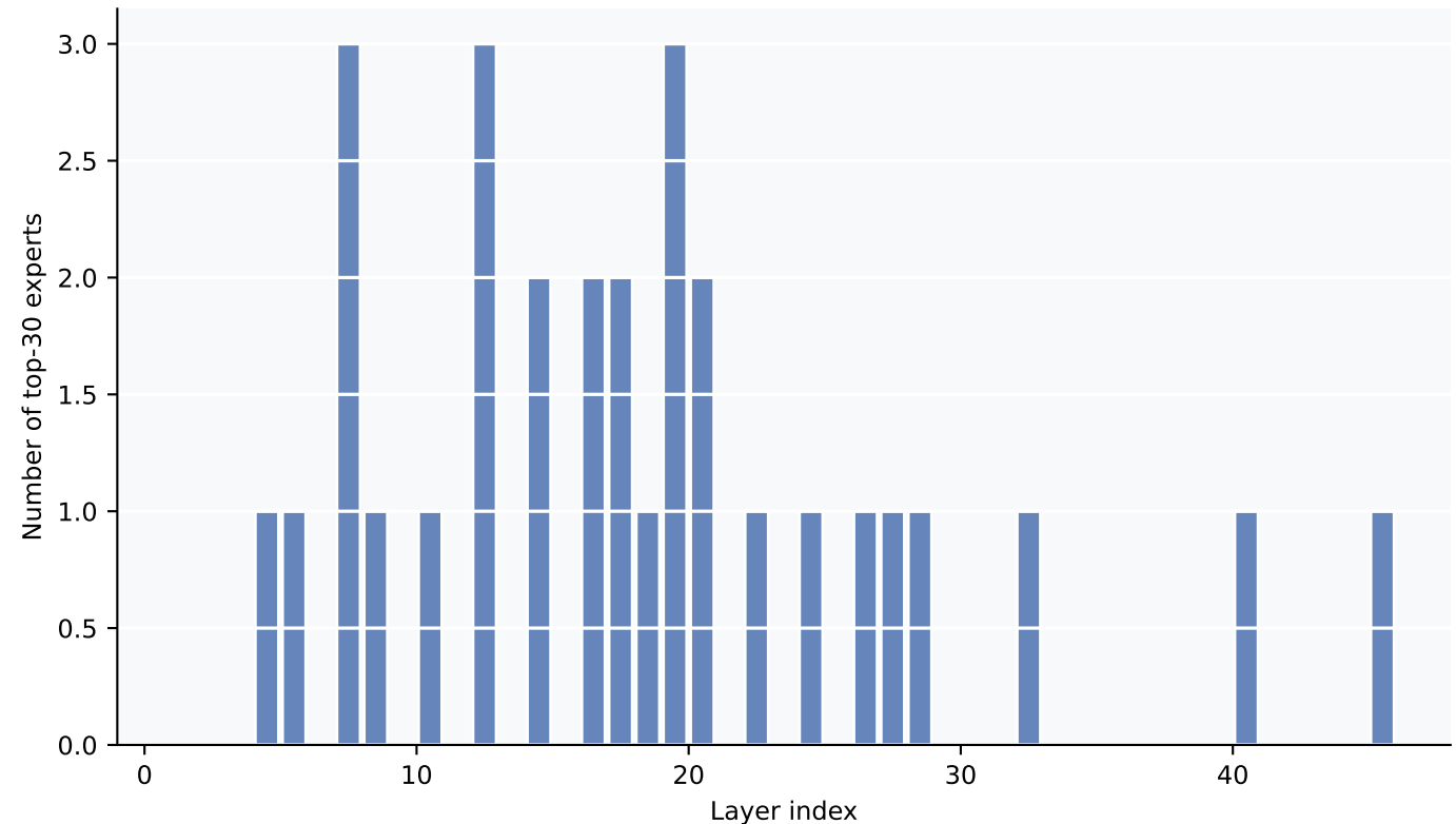
Layer Distribution — Top-30 Global Spatial Experts
