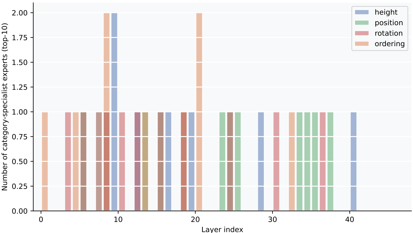
Layer Distribution — Per-Category Top-10 Specialist Experts
