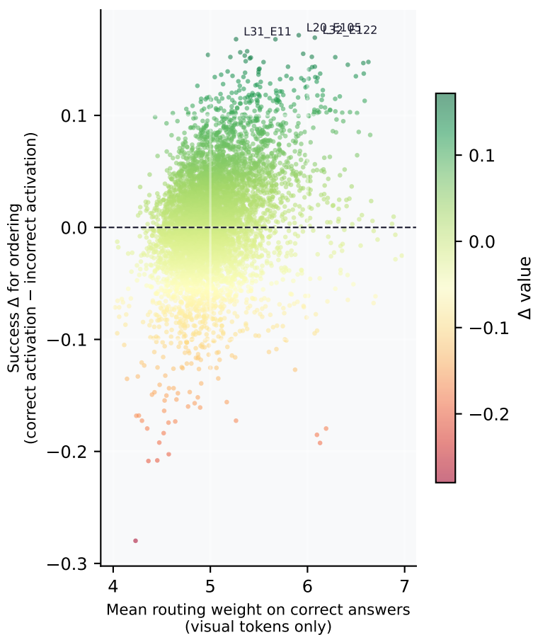
ORDERING
