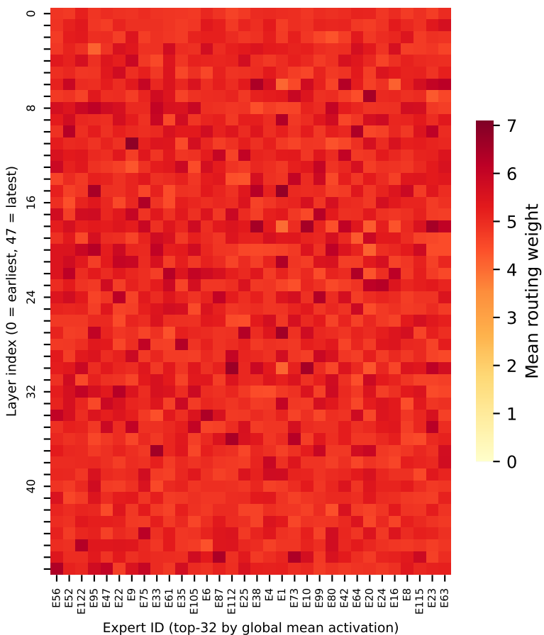
ROTATION (acc=24.0%)
