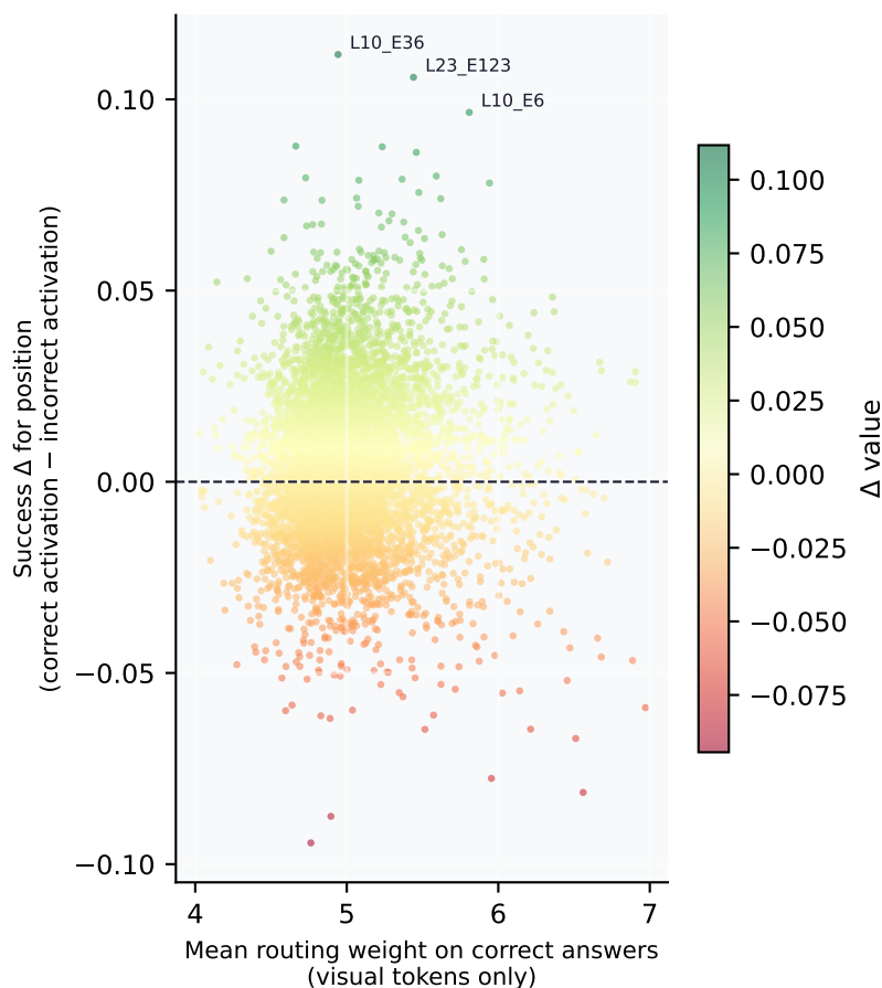
ORDERING
