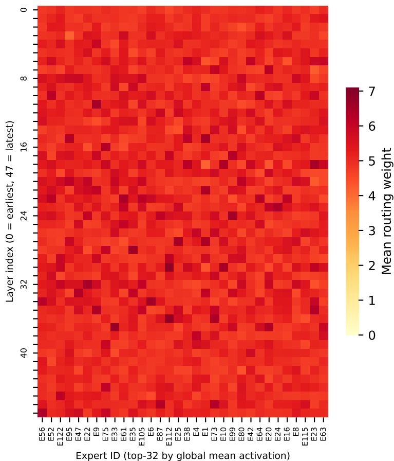
ORDERING (acc=20.0%)
