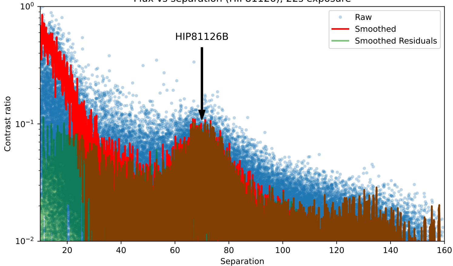
Flux vs separation (HIP81126), 22s exposure
