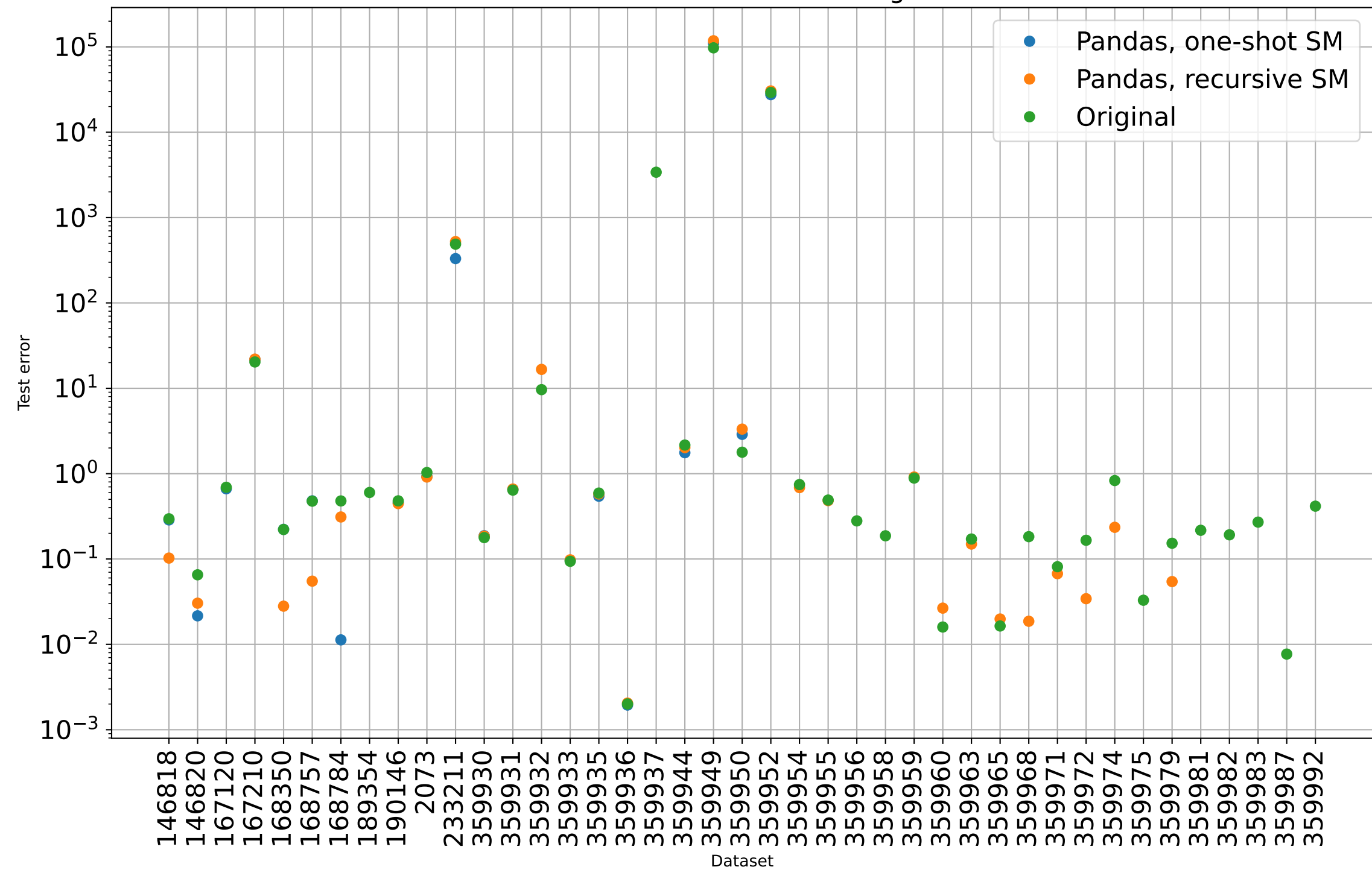
Test error of the model on the feature-engineered datasets
