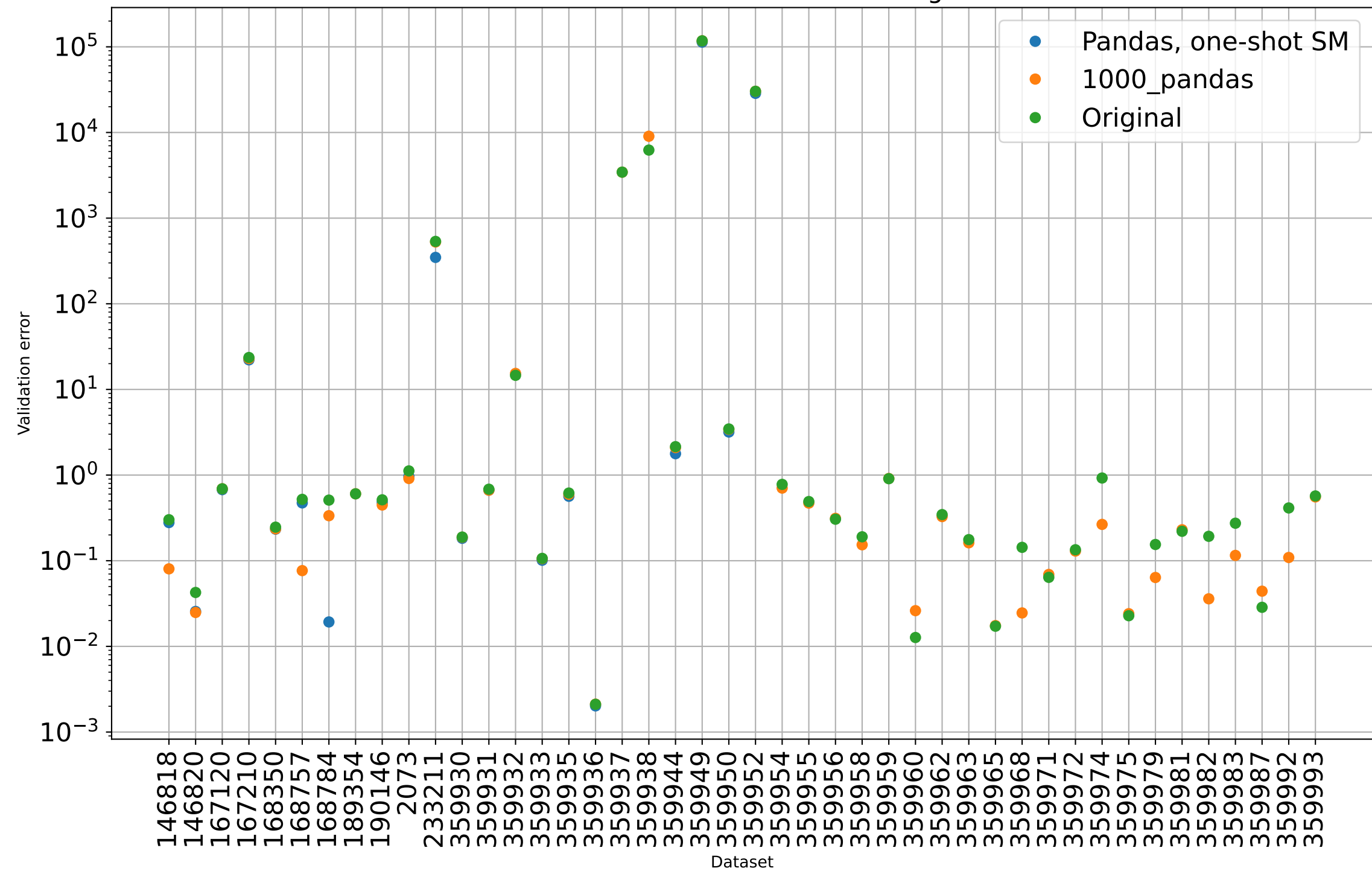
Validation error of the model on the feature-engineered datasets
