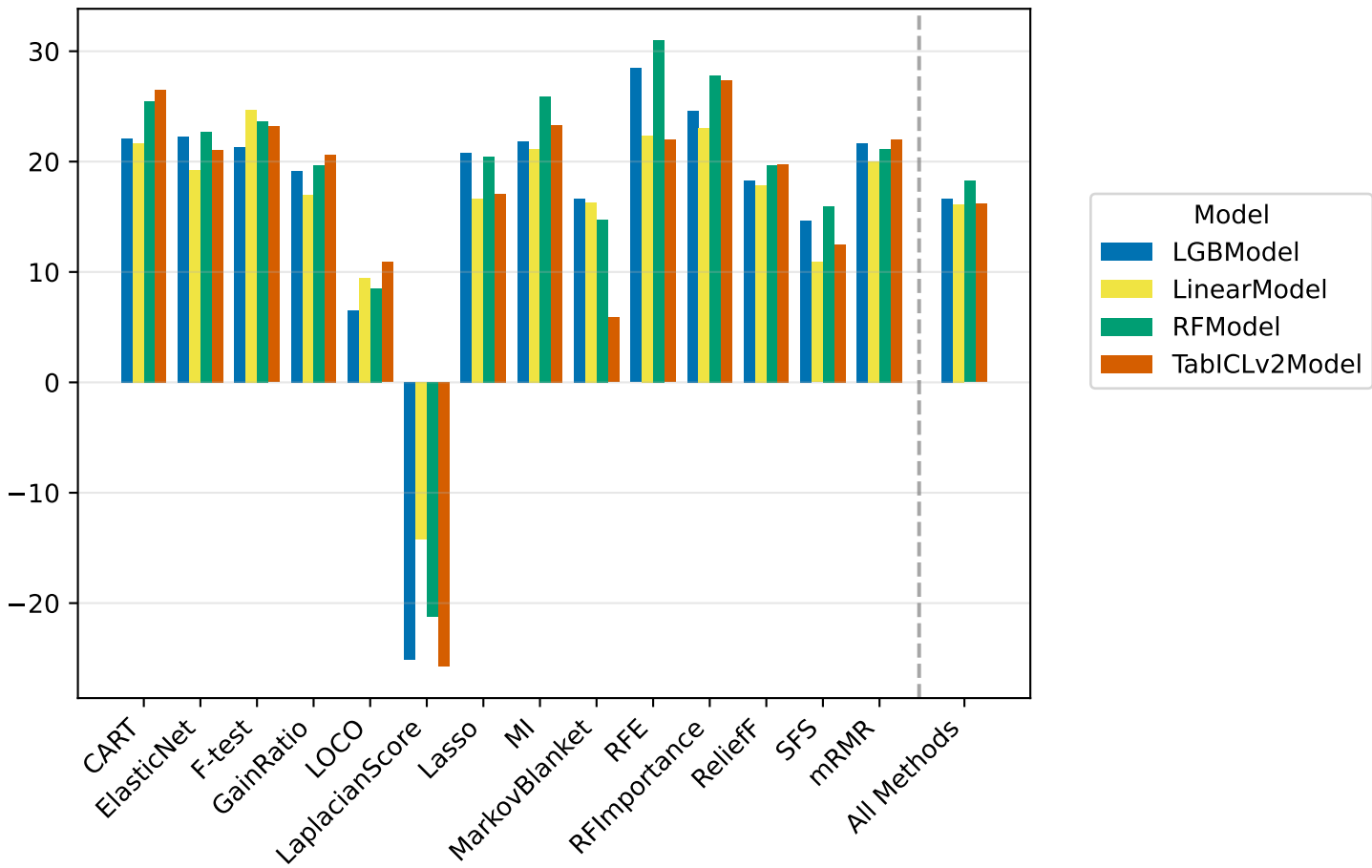
Improvement over Random (%)
