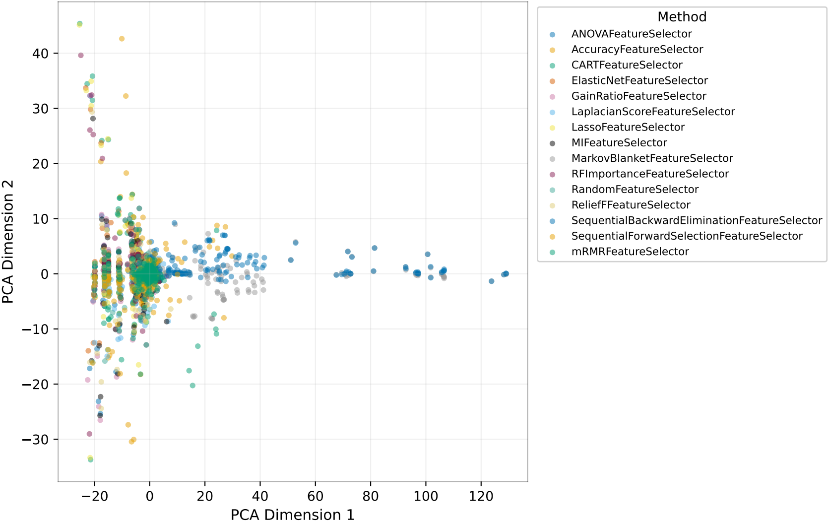
PCA of Feature Selection Vectors (per dataset×budget)
