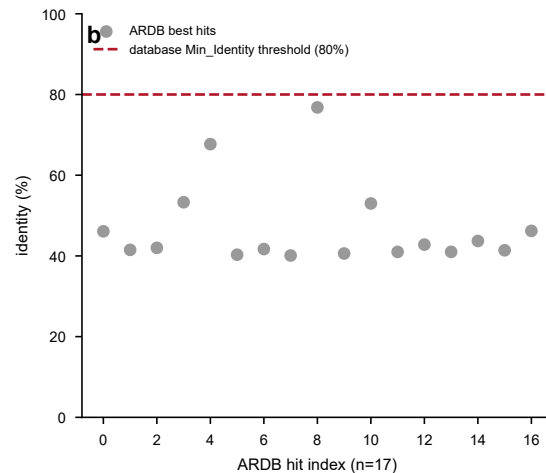
b ARDB hits are below the database threshold
