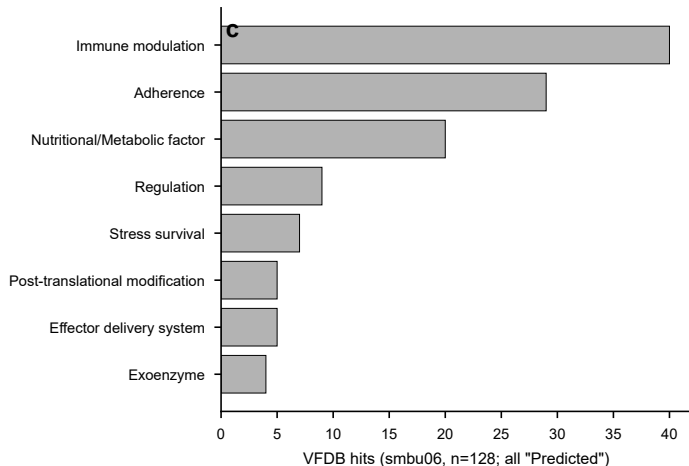
c VFDB category counts
