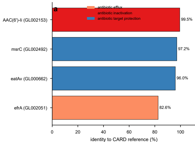
a CARD strict hits (4 genes, both strains)
