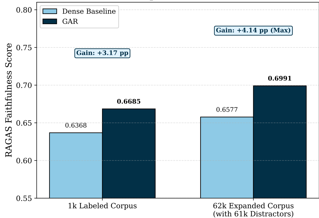
(b) Faithfulness Gain Amplification Under Distractor Scaling
