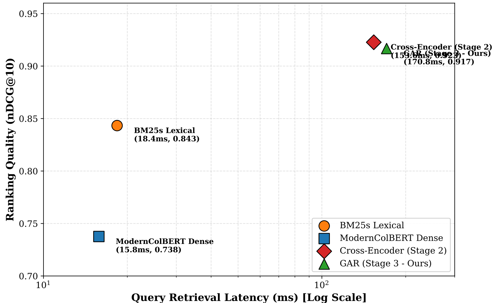
Latency vs. Ranking Accuracy Trade-Off on 62k Corpus
