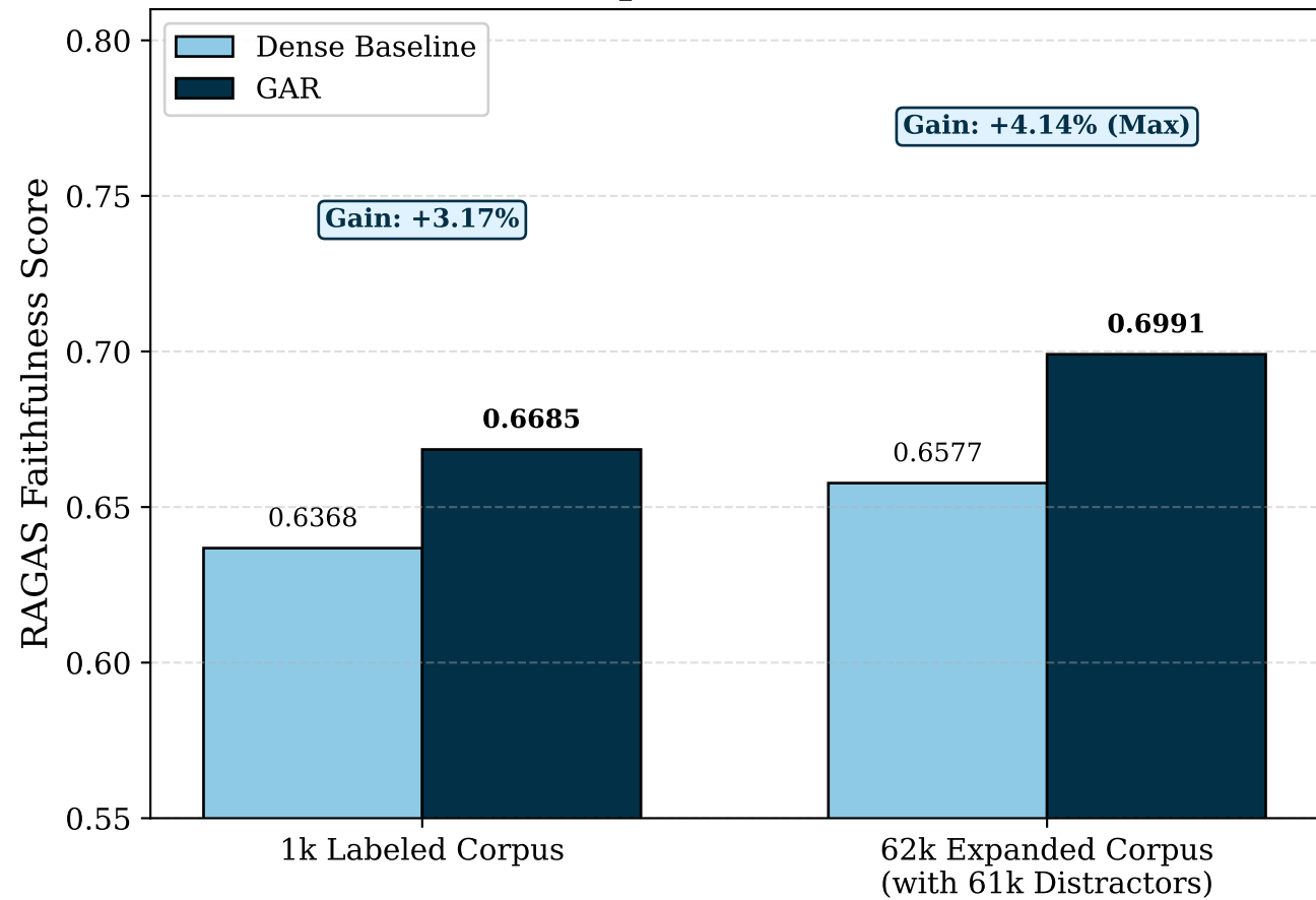
(b) Faithfulness Gain Amplification Under Distractor Scaling
