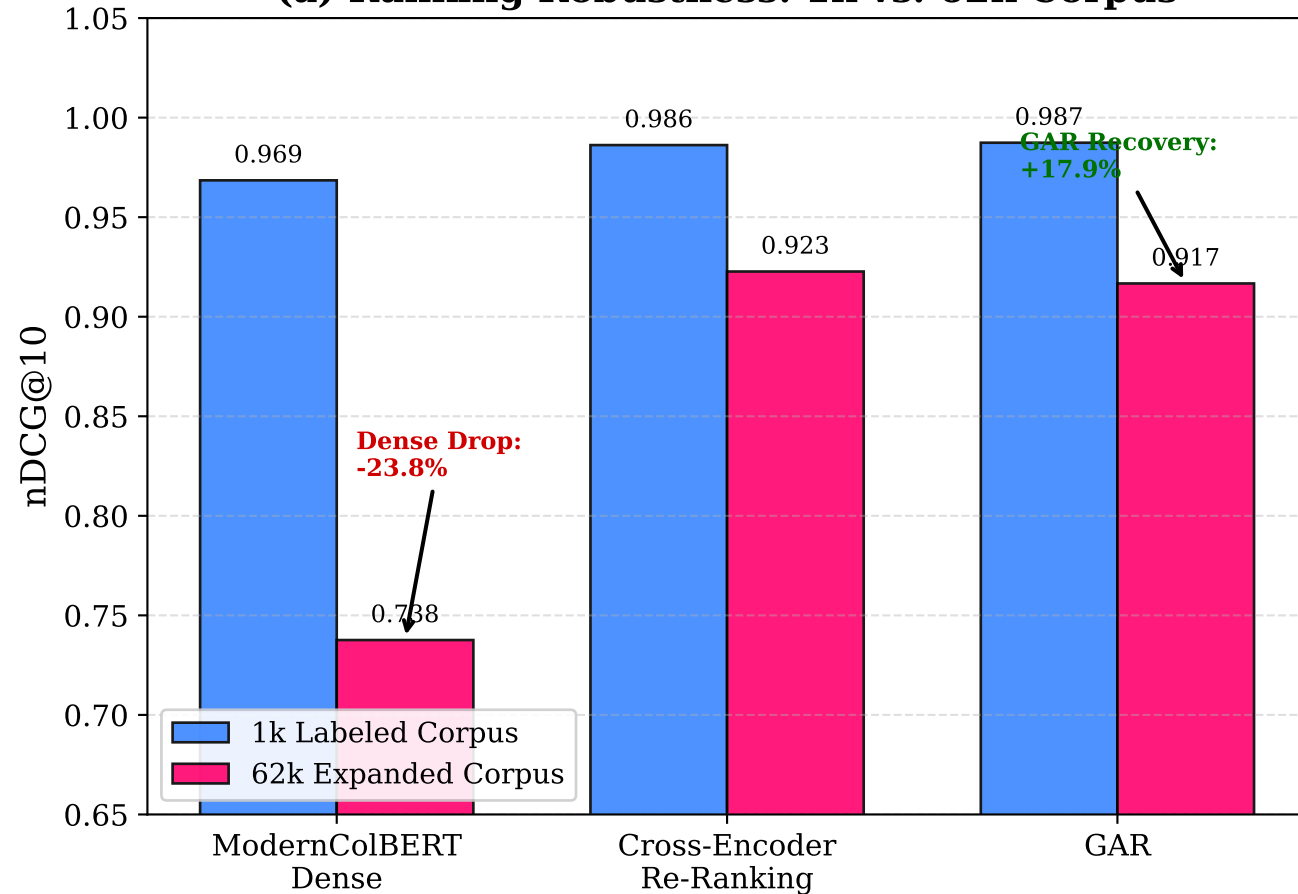
(a) Ranking Robustness: 1k vs. 62k Corpus
