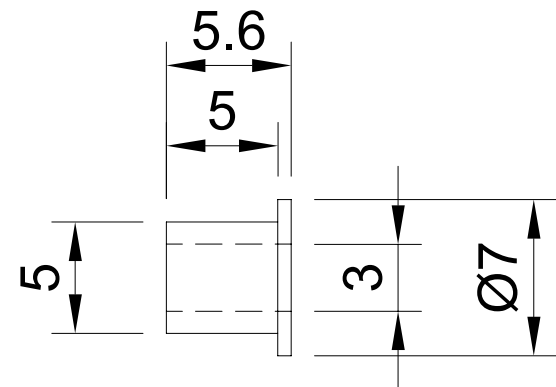
Shoulder Bushing
