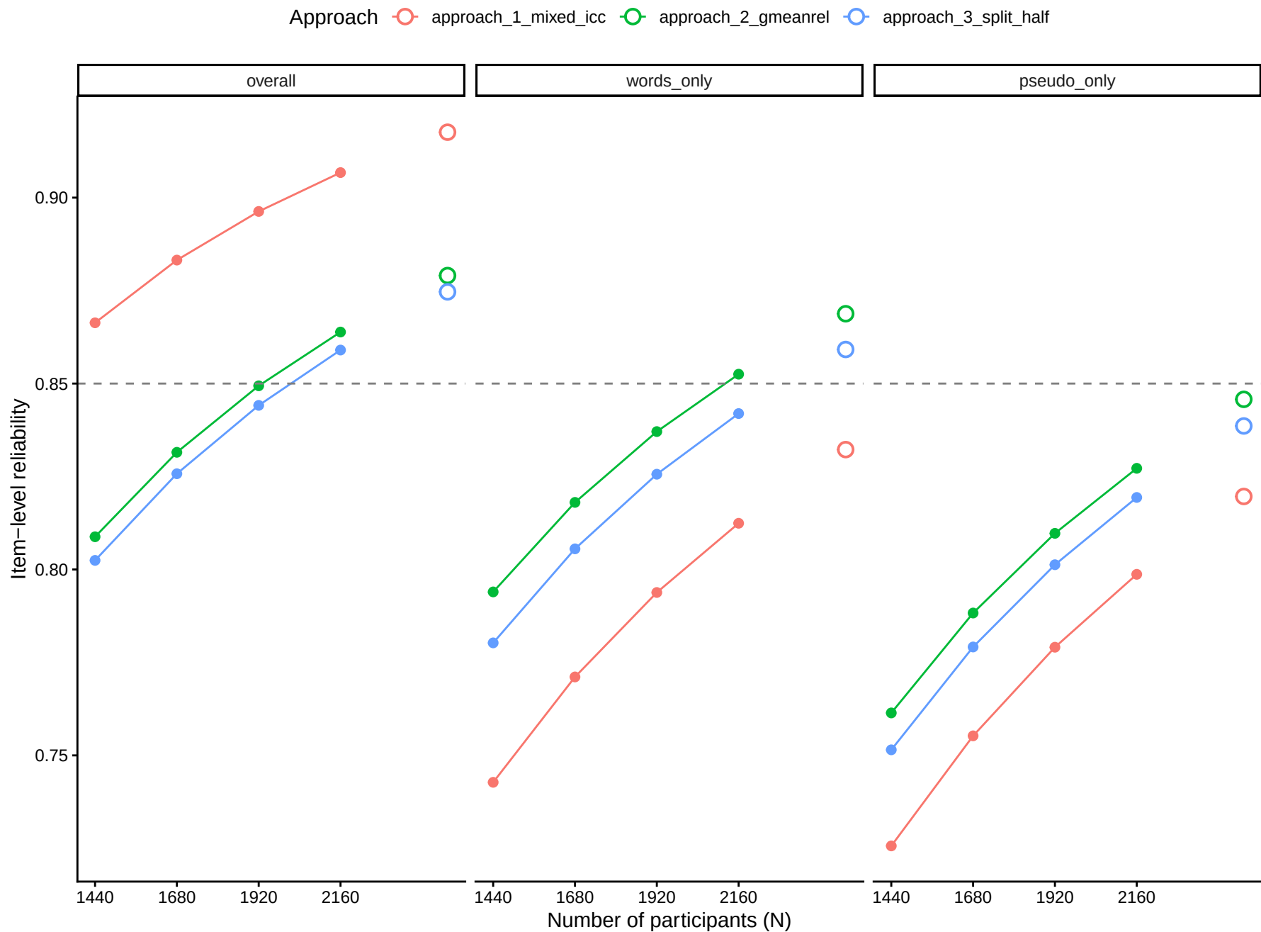
Current reliability and Spearman–Brown projections (3 approaches × 3 conditions)
