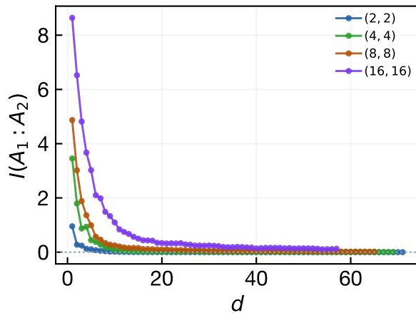
(b) Hyperbolic \{3, 7\} , L = 147 , \mu = 0.1
