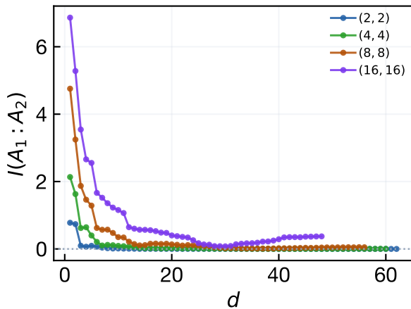
(a) Periodic MERA, L = 128 , \mu = 0.1
